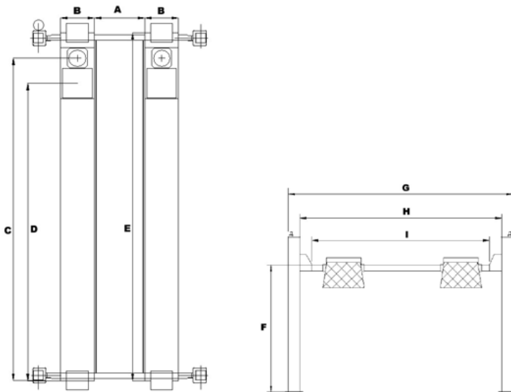
Dimensions (mm)
